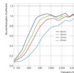
Reverberation Tube
